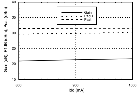
Gain & Power vs. Supply Current @ 38 GHz
